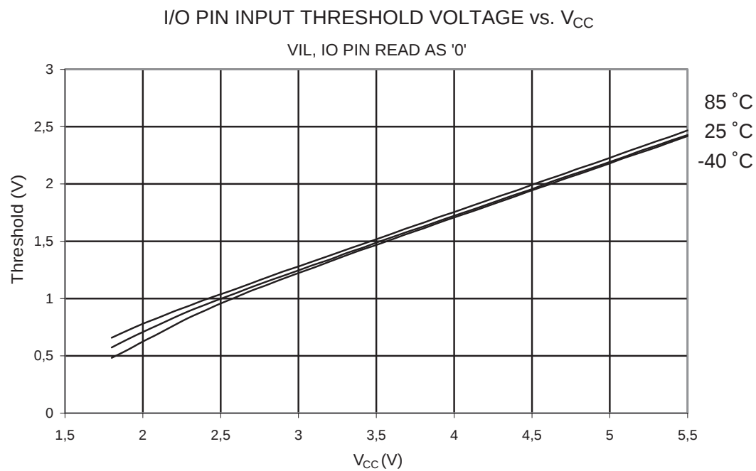
Figure 20-28. I/O Pin Input Threshold Voltage vs. V_{CC} ( V_{IL} , I/O Pin Read as '0')
