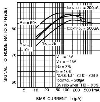
Fig.10 SN ratio vs. diode bias current
