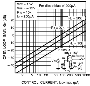
Fig.6 Open loop gain control current characteristics
