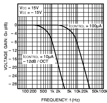
Fig.13 Secondary low pass filter characteristics
