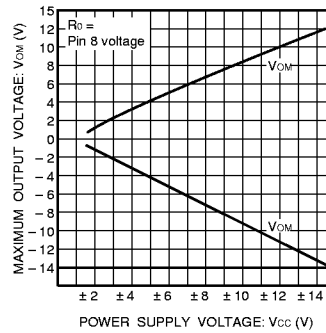
Fig.11 Maximum output voltage vs. power supply voltage
