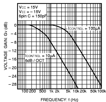
Fig.12 Low pass filter characteristics
