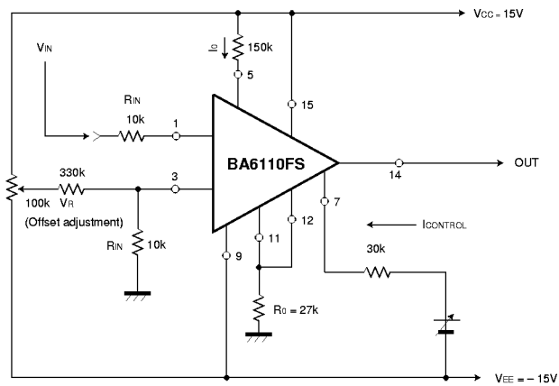
Fig.3 Voltage-controlled amplifier (electronic volume control)
