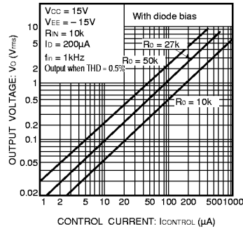
Fig.7 THD 0.5% output control current characteristics
