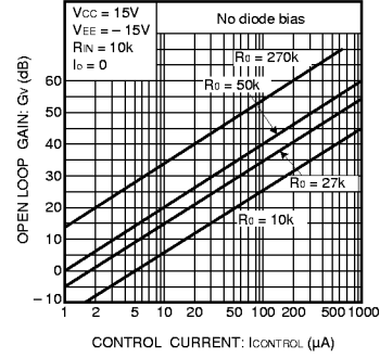
Fig.8 Open loop gain control current characteristics
