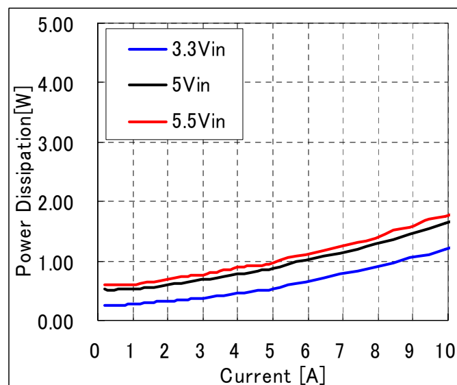
Fig-2.5V-3: Power dissipation vs. load current and input voltage for V_{out}=2.5V . Airflow rate=200 LFM (1.0m/s) and T_a=25^{\circ}C .
