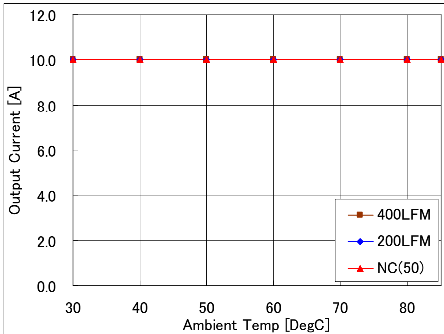
Fig-2.0V-1: Available load current vs. ambient temperature and airflow rates for V_{out}=2.0V with V_{in}=5.0V . Maximum component temperature \leq 120^{\circ}C
