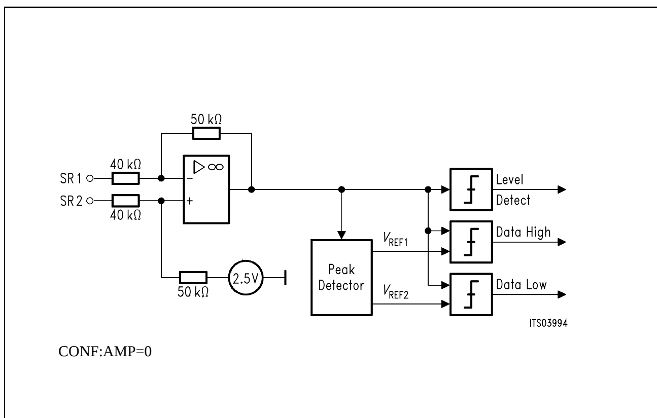
Figure 29 Receiver Circuit
