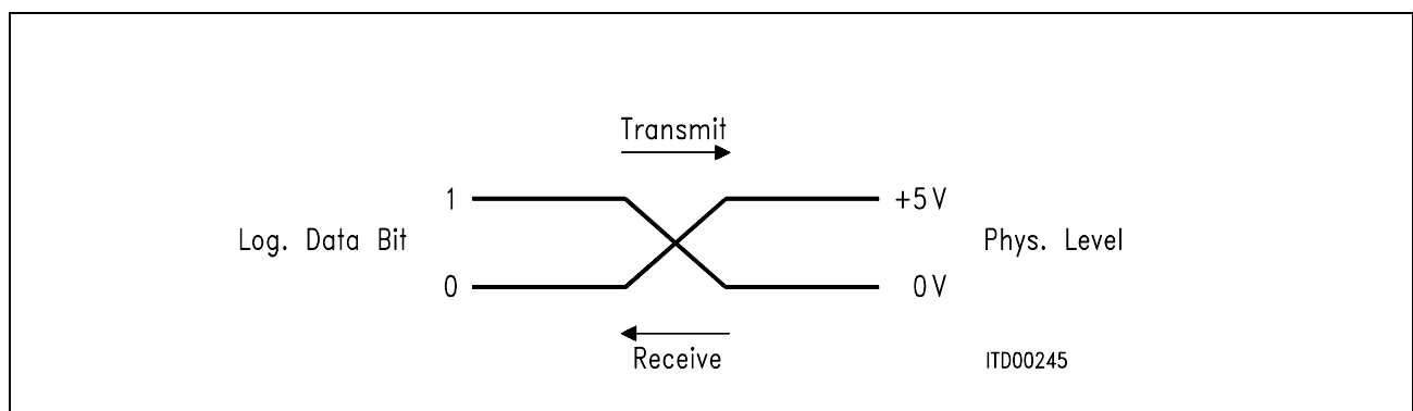
Figure 13 Data Inversion
