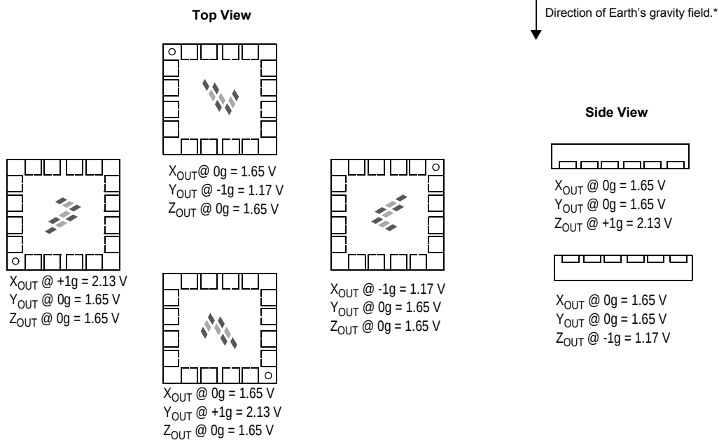
Figure 19. Orientation and Output Values for MMA7261QT
