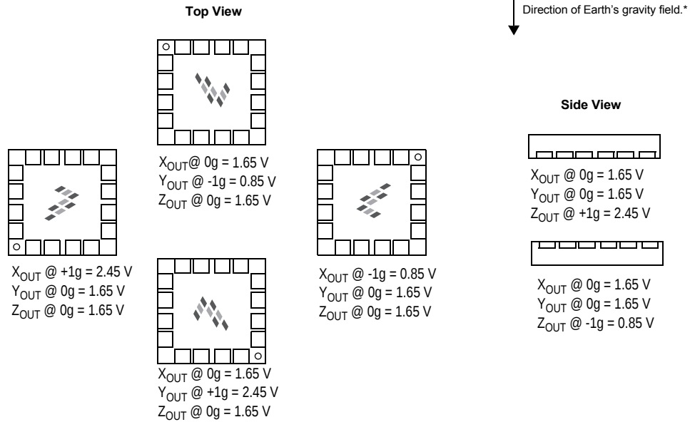
Figure 18. Orientation and Output Values for MMA7260QT, MMA6270QT and MMA6280QT
