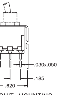
PRINTED CIRCUIT MOUNTING
