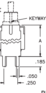
FRONT VIEW DOUBLE POLE
