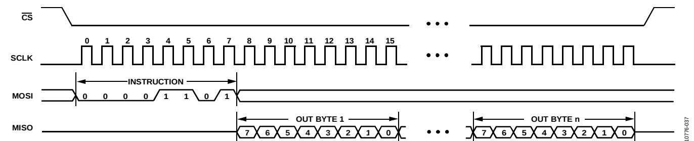
Figure 40. FIFO Read
