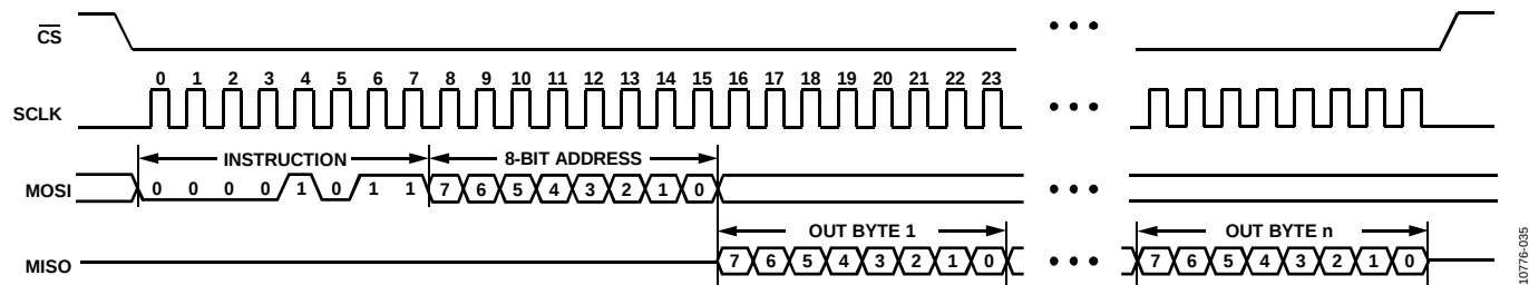
Figure 38. Burst Read
