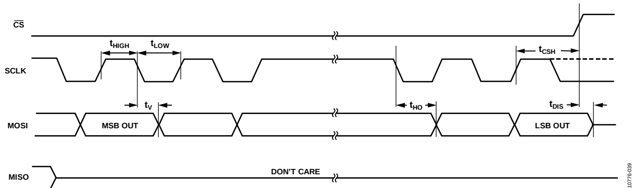
Figure 42. Timing Diagram for SPI Read Instructions
