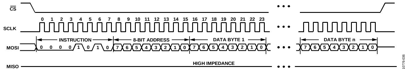
Figure 39. Burst Write
