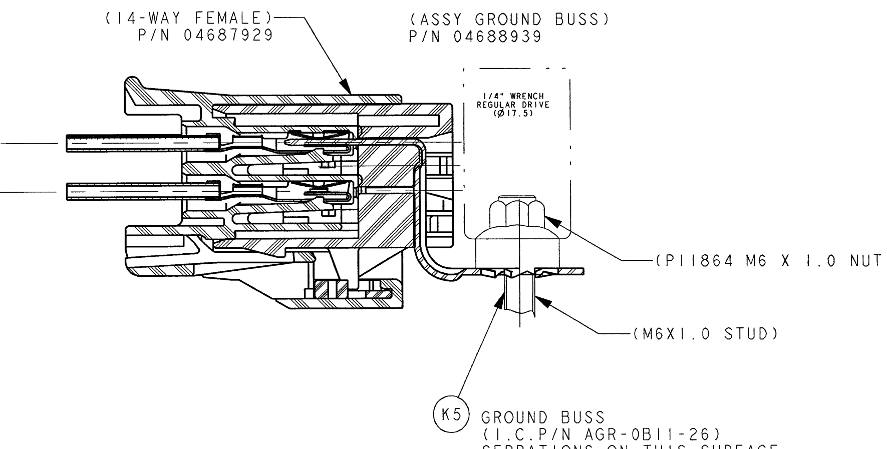
ASSY VIEW FOR REF P/N 04688939 & 04687929
