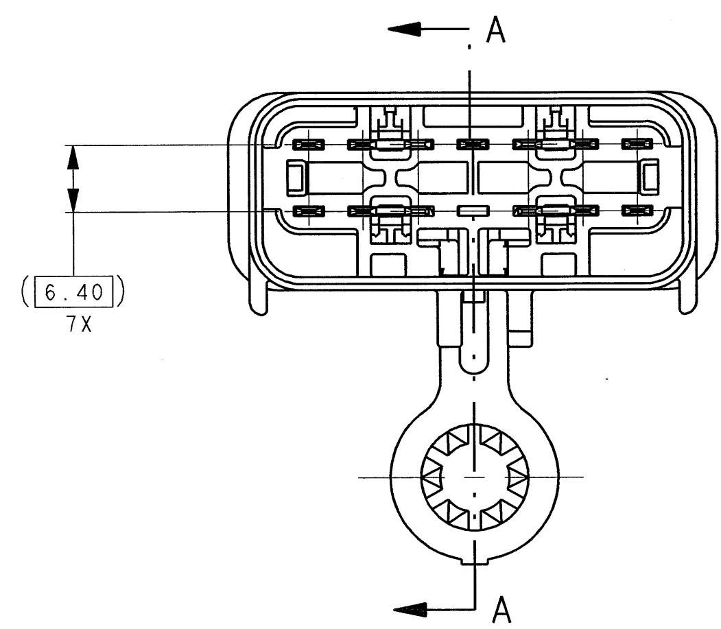
ASSY GROUND BUSS 90° P/N 04707084
