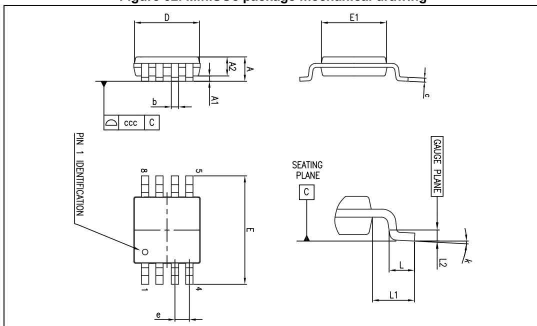
Figure 32. MiniSO8 package mechanical drawing
