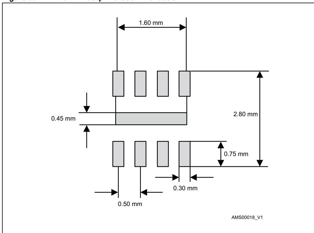
Figure 30. DFN8 2x2 footprint recommendation
