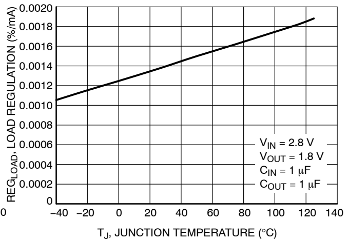
Figure 8. Load Regulation vs. Temperature – V_{OUT} = 1.8 V
