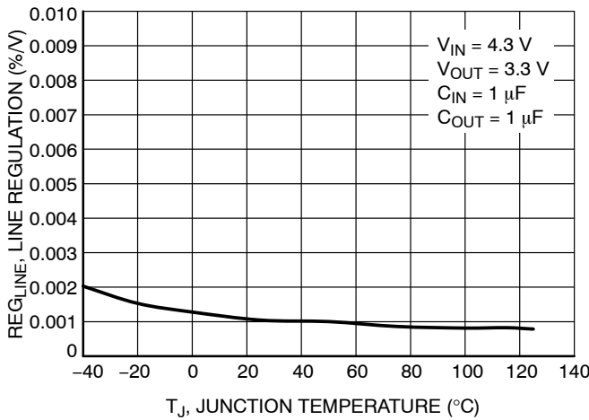
Figure 7. Line Regulation vs. Temperature – V_{OUT} = 3.3 V
