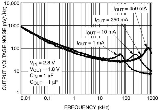
Figure 22. Output Voltage Noise Spectral Density – V_{OUT} = 1.8 V
