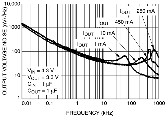
Figure 23. Output Voltage Noise Spectral Density – V_{OUT} = 3.3 V
