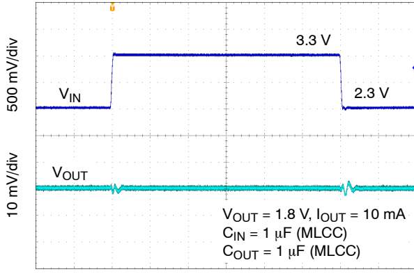
Figure 30. Line Transient Response – V_{OUT} = 1.8\text{ V}
