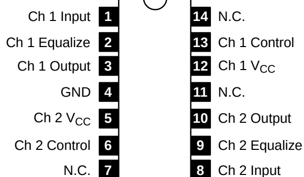
Pin Connection Diagram
