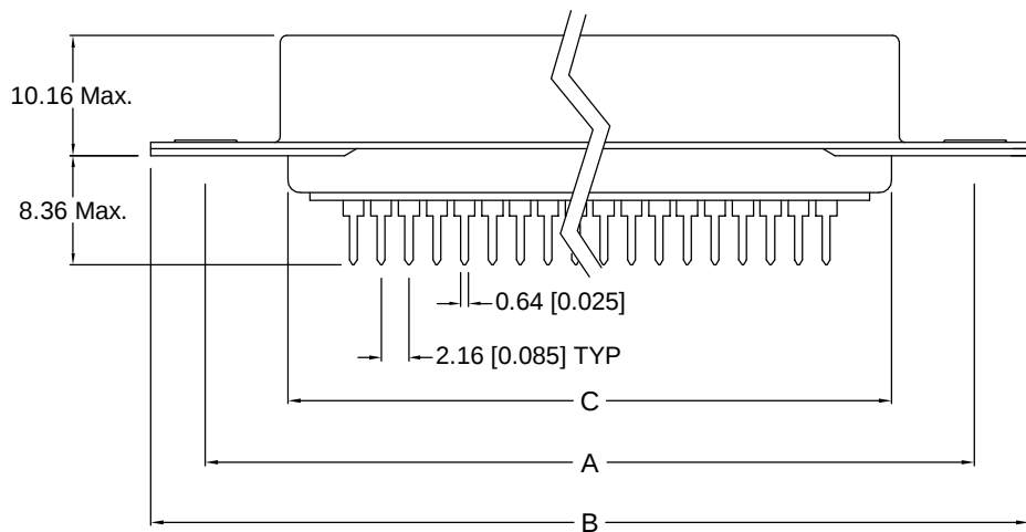
Receptacles Without Spring Latch Dimensions mm/in.
