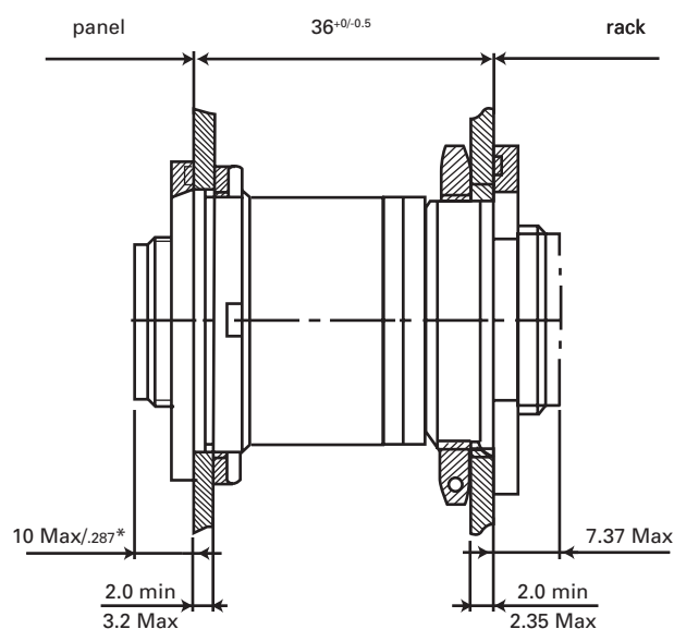
Mated connectors plug (type 26) and receptacle (type 27)
