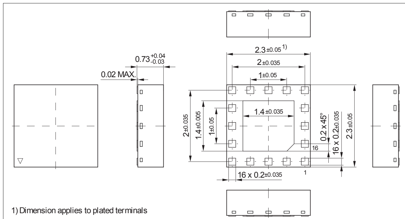
Figure 3 Package Outline
