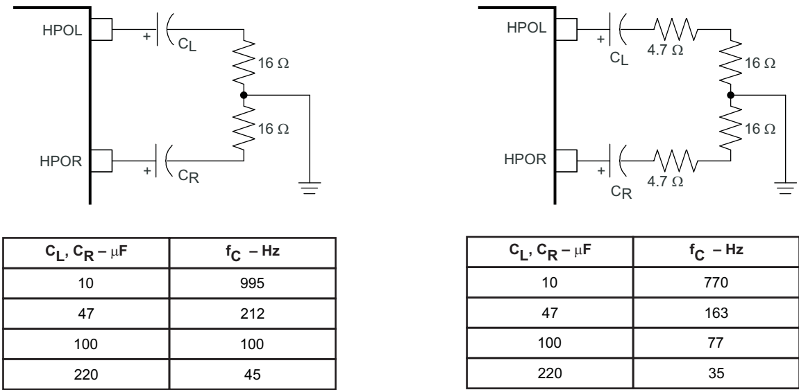
Figure 43. High-Pass Filter for Headphone Output
