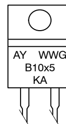
TO-220AC CASE 221B PLASTIC
