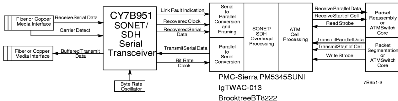
Figure 1. SONET/SDH and ATM Interface
