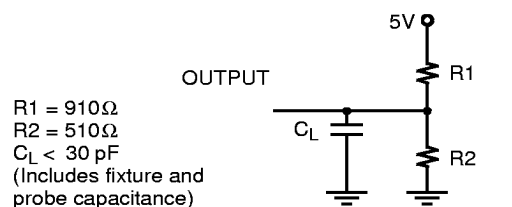
(a) TTL AC Test Load [7]
