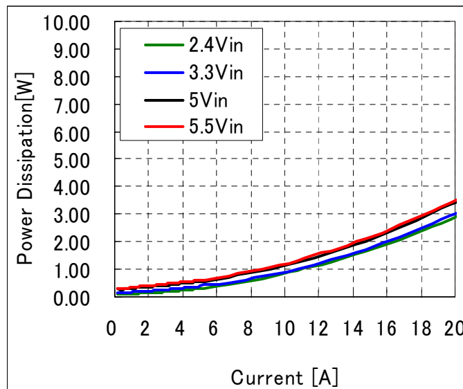
Fig-1.2V-3: Power dissipation vs. load current and input voltage for Vout=1.2V. Airflow rate=200 LFM (1.0m/s) and Ta=25°C.
