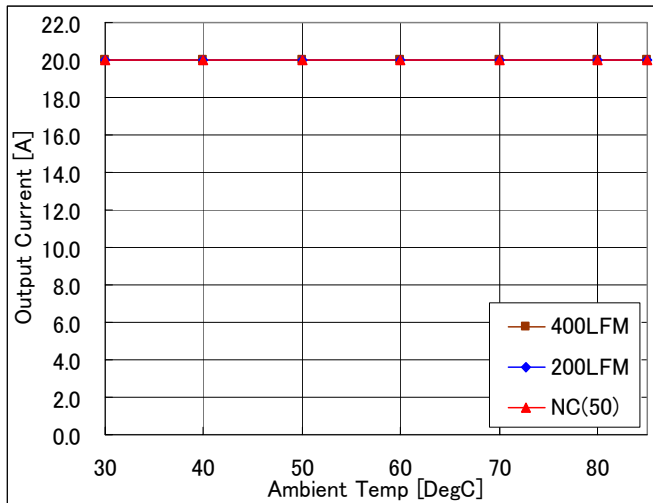
Fig-0.7525V-1a: Available load current vs. ambient temperature and airflow rates for V_{out}=0.7525V with V_{in}=5.0V . Maximum component temperature \leq 120^{\circ}C
