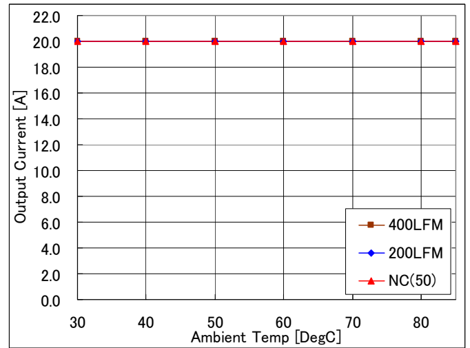
Fig-1.8V-1b: Available load current vs. ambient temperature and airflow rates for Vout=1.8V with Vin=5.0V. Maximum component temperature \leq 120^{\circ}\text{C}
