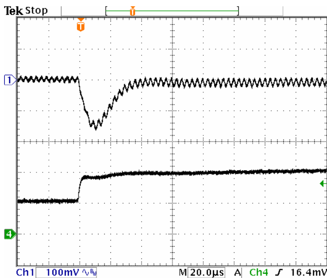
Fig-1.2V-6: Output voltage response for Vout=1.2V to positive load current step-change from 10A to 20A with slew rate of 5A/ \mu s at Vin=5.0V. Co=47 \mu Fx4 ceramic.
