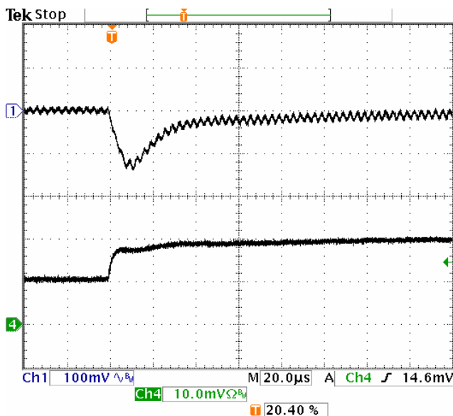
Fig-0.7525V-6: Output voltage response for V_{out}=0.7525V to positive load current step-change from 10A to 20A with slew rate of 5A/\mu s at V_{in}=5.0V . C_o=47\mu F \times 4 ceramic.
