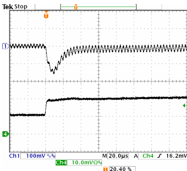
Fig-2.0V-6: Output voltage response for V_{out}=2.0V to positive load current step-change from 10A to 20A with slew rate of 5A/\mu s at V_{in}=5.0V . C_o=47\mu F \times 4 ceramic.
