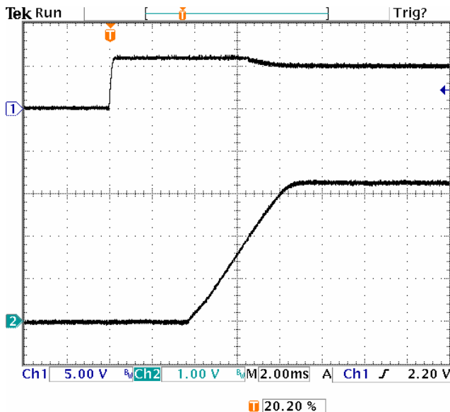
Fig-3.3V-4: Turn-on transient for Vout=3.3V with application of Vin at full rated load current (resistive) and 47 \mu Fx4 external capacitance at Vin=5.0V.
