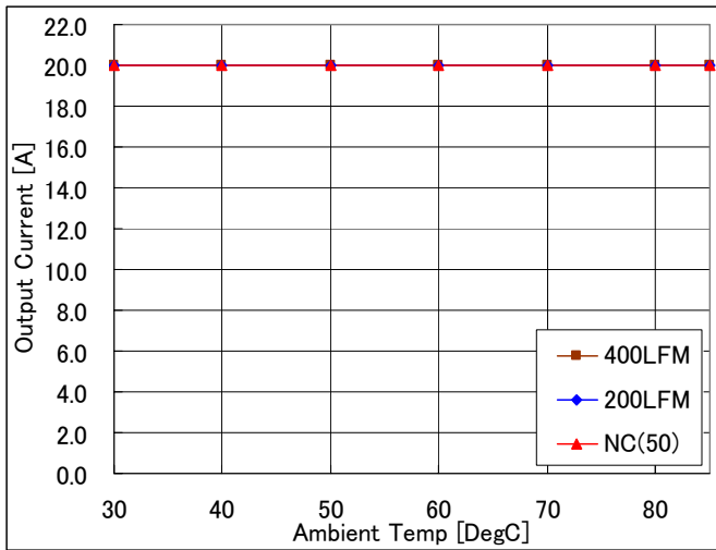
Fig-1.0V-1a: Available load current vs. ambient temperature and airflow rates for Vout=1.0V with Vin=5.0V. Maximum component temperature \leq 120^{\circ}\text{C}
