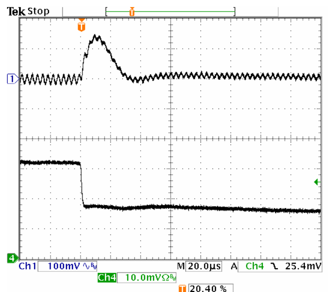
Fig-2.0V-7: Output voltage response for V_{out}=2.0V to positive load current step-change from 20A to 10A with slew rate of -5A/\mu s at V_{in}=5.0V . C_o=47\mu F \times 4 ceramic.
