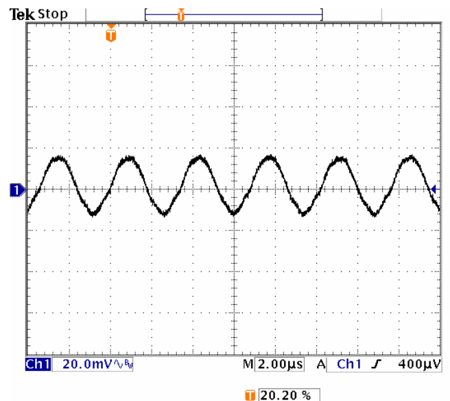
Fig-1.5V-5: Output voltage ripple (20mV/div.) for Vout=1.5V at full rated load current into a resistive load with external capacitance 47 \mu Fx4 ceramic + 1 \mu F ceramic at Vin=5.0V.
