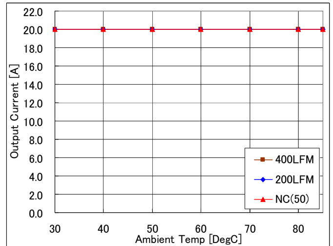
Fig-2.5V-1b: Available load current vs. ambient temperature and airflow rates for Vout=2.5V with Vin=5.0V. Maximum component temperature \leq 120^{\circ}\text{C}
