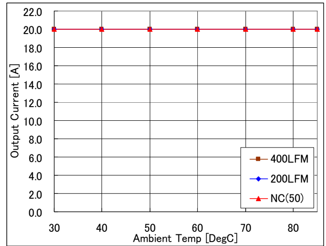
Fig-1.0V-1b: Available load current vs. ambient temperature and airflow rates for Vout=1.0V with Vin=5.0V. Maximum component temperature \leq 120^{\circ}\text{C}
