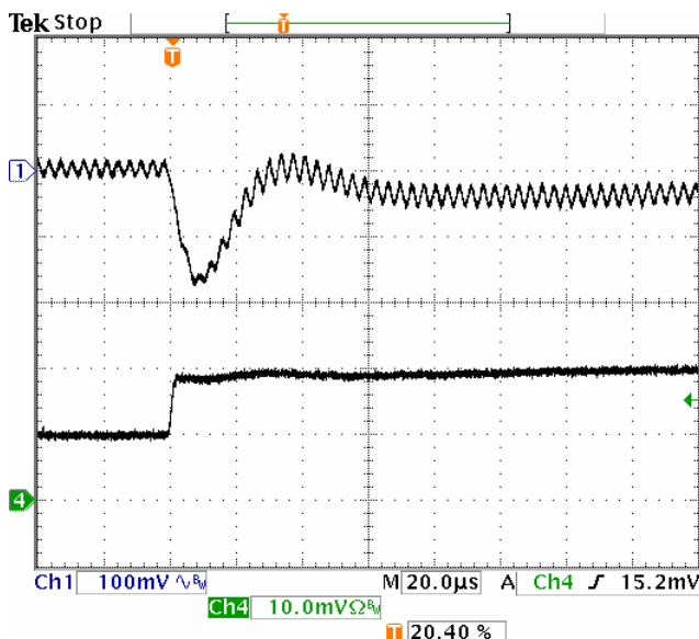
Fig-3.3V-6: Output voltage response for Vout=3.3V to positive load current step-change from 10A to 20A with slew rate of 5A/ \mu s at Vin=5.0V. Co=47 \mu Fx4 ceramic.
