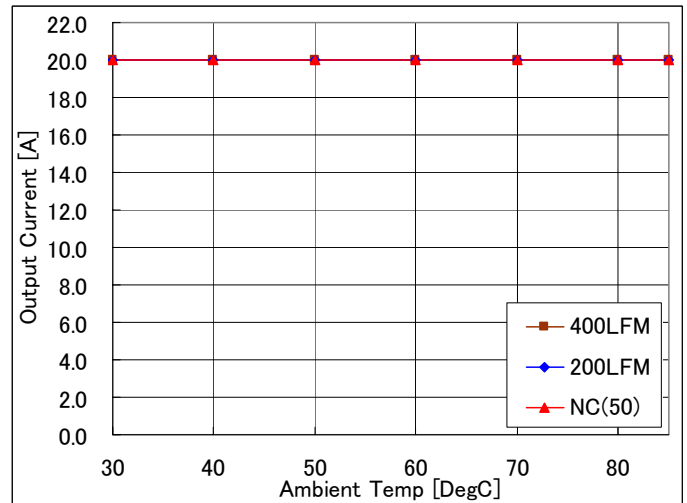
Fig-0.7525V-1b: Available load current vs. ambient temperature and airflow rates for V_{out}=0.7525V with V_{in}=5.0V . Maximum component temperature \leq 120^{\circ}C
