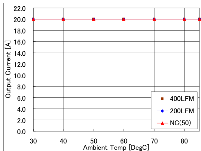
Fig-1.2V-1b: Available load current vs. ambient temperature and airflow rates for Vout=1.2V with Vin=5.0V. Maximum component temperature \leq 120^{\circ}\text{C}
