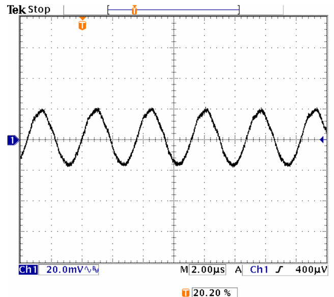
Fig-3.3V-5: Output voltage ripple (20mV/div.) for Vout=3.3V at full rated load current into a resistive load with external capacitance 47 \mu Fx4 ceramic + 1 \mu F ceramic at Vin=5.0V.
