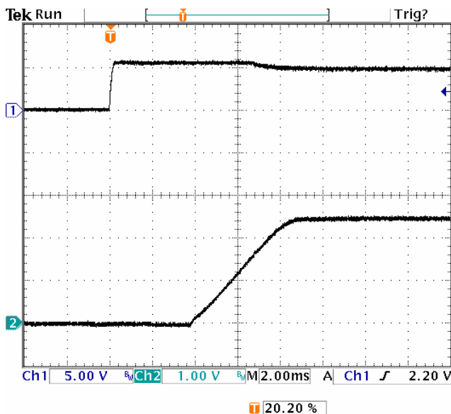
Fig-2.5V-4: Turn-on transient for Vout=2.5V with application of Vin at full rated load current (resistive) and 47 \mu Fx4 external capacitance at Vin=5.0V.
