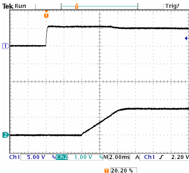
Fig-1.5V-4: Turn-on transient for Vout=1.5V with application of Vin at full rated load current (resistive) and 47 \mu Fx4 external capacitance at Vin=5.0V.
