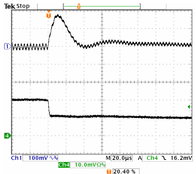
Fig-1.5V-7: Output voltage response for Vout=1.5V to positive load current step-change from 20A to 10A with slew rate of -5A/ \mu s at Vin=5.0V. Co=47 \mu Fx4 ceramic.
