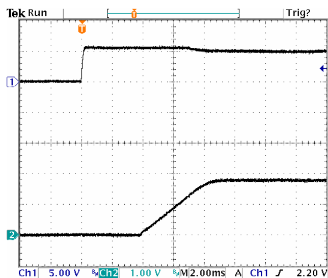
Fig-1.8V-4: Turn-on transient for Vout=1.8V with application of Vin at full rated load current (resistive) and 47 \mu Fx4 external capacitance at Vin=5.0V.
