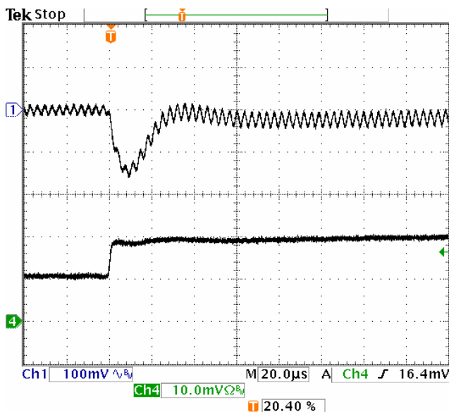
Fig-2.5V-6: Output voltage response for Vout=2.5V to positive load current step-change from 10A to 20A with slew rate of 5A/ \mu s at Vin=5.0V. Co=47 \mu Fx4 ceramic.
