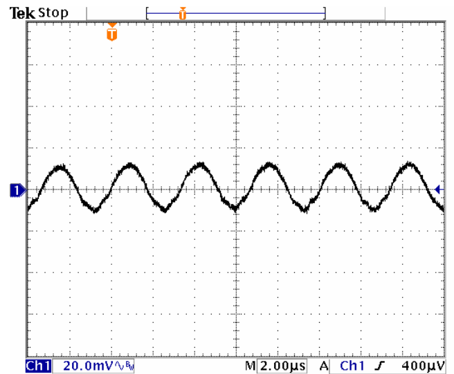
Fig-1.2V-5: Output voltage ripple (20mV/div.) for Vout=1.2V at full rated load current into a resistive load with external capacitance 47 \mu Fx4 ceramic + 1 \mu F ceramic at Vin=5.0V.
