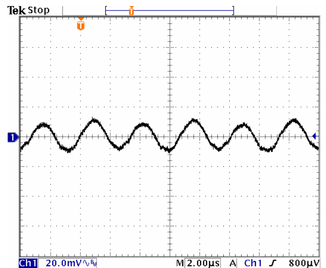
Fig-1.0V-5: Output voltage ripple (20mV/div.) for Vout=1.0V at full rated load current into a resistive load with external capacitance 47 \mu Fx4 ceramic + 1 \mu F ceramic at Vin=5.0V.
