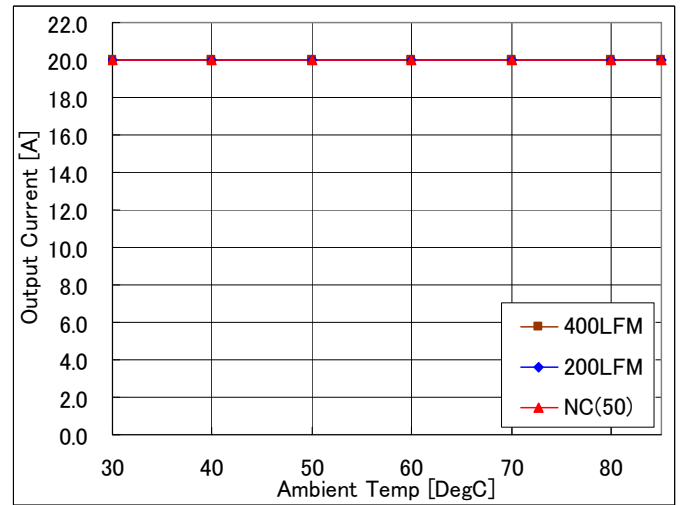
Fig-3.3V-1b: Available load current vs. ambient temperature and airflow rates for V_{out}=3.3V with V_{in}=5.0V . Maximum component temperature \leq 120^{\circ}C
