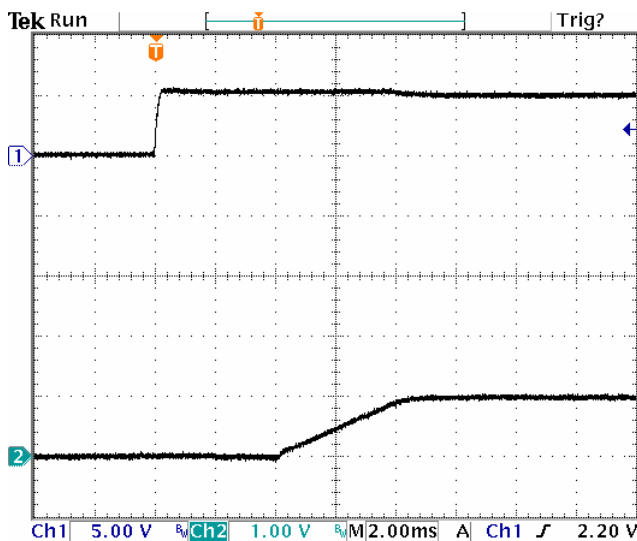
Fig-1.0V-4: Turn-on transient for Vout=1.0V with application of Vin at full rated load current (resistive) and 47 \mu Fx4 external capacitance at Vin=5.0V.
