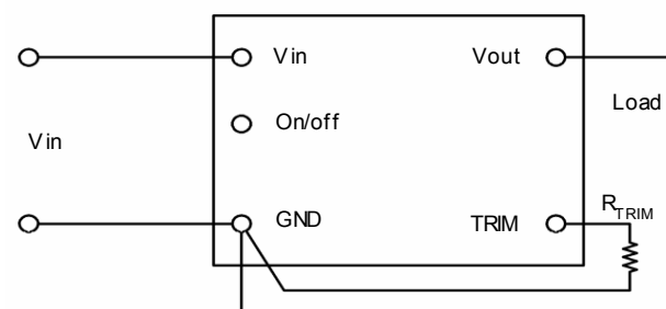
Fig. C: Configuration for programming output voltage
