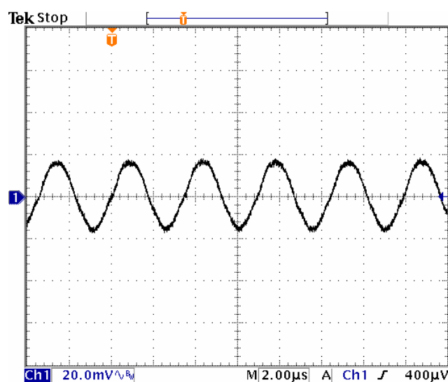
Fig-1.8V-5: Output voltage ripple (20mV/div.) for Vout=1.8V at full rated load current into a resistive load with external capacitance 47 \mu Fx4 ceramic + 1 \mu F ceramic at Vin=5.0V.
