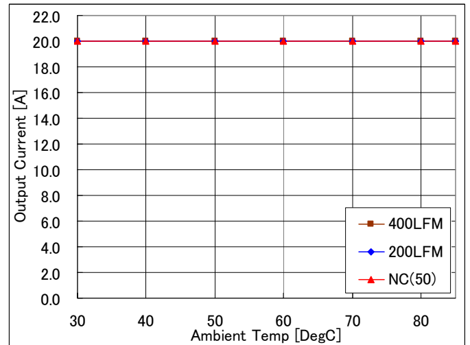
Fig-1.5V-1b: Available load current vs. ambient temperature and airflow rates for Vout=1.5V with Vin=5.0V. Maximum component temperature \leq 120^{\circ}\text{C}
