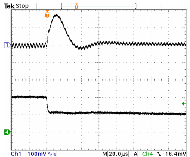
Fig-1.2V-7: Output voltage response for Vout=1.2V to positive load current step-change from 20A to 10A with slew rate of -5A/ \mu s at Vin=5.0V. Co=47 \mu Fx4 ceramic.
