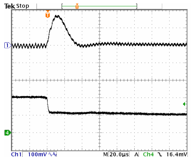
Fig-1.0V-7: Output voltage response for Vout=1.0V to positive load current step-change from 20A to 10A with slew rate of -5A/ \mu s at Vin=5.0V. Co=47 \mu Fx4 ceramic.
