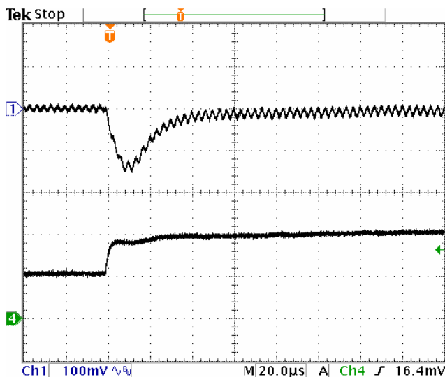
Fig-1.0V-6: Output voltage response for Vout=1.0V to positive load current step-change from 10A to 20A with slew rate of 5A/ \mu s at Vin=5.0V. Co=47 \mu Fx4 ceramic.
