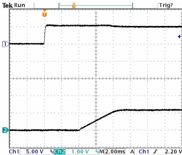
Fig-1.2V-4: Turn-on transient for Vout=1.2V with application of Vin at full rated load current (resistive) and 47 \mu Fx4 external capacitance at Vin=5.0V.
