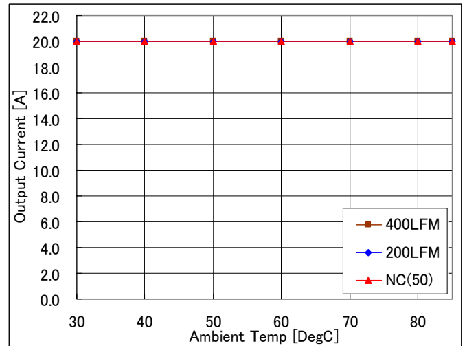
Fig-2.0V-1b: Available load current vs. ambient temperature and airflow rates for V_{out}=2.0V with V_{in}=5.0V . Maximum component temperature \leq 120^{\circ}C
