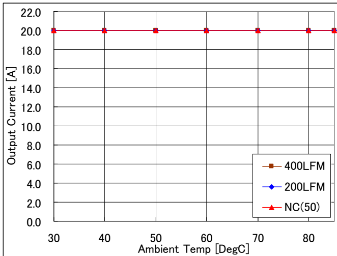
Fig-2.5V-1a: Available load current vs. ambient temperature and airflow rates for Vout=2.5V with Vin=5.0V. Maximum component temperature \leq 120^{\circ}\text{C}
