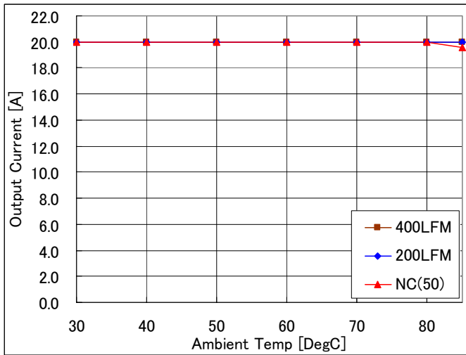
Fig-3.3V-1a: Available load current vs. ambient temperature and airflow rates for V_{out}=3.3V with V_{in}=5.0V . Maximum component temperature \leq 120^{\circ}C
