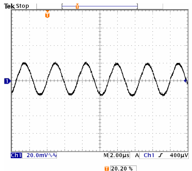
Fig-2.5V-5: Output voltage ripple (20mV/div.) for Vout=2.5V at full rated load current into a resistive load with external capacitance 47 \mu Fx4 ceramic + 1 \mu F ceramic at Vin=5.0V.
