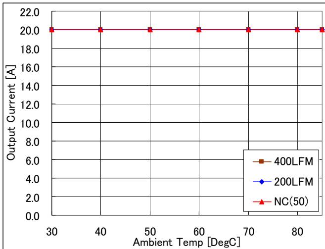
Fig-2.0V-1a: Available load current vs. ambient temperature and airflow rates for V_{out}=2.0V with V_{in}=5.0V . Maximum component temperature \leq 120^{\circ}C
