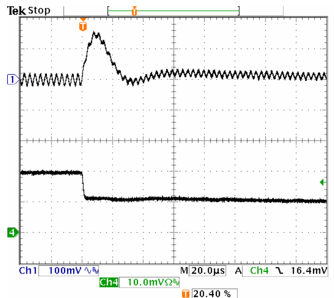
Fig-2.5V-7: Output voltage response for Vout=2.5V to positive load current step-change from 20A to 10A with slew rate of -5A/ \mu s at Vin=5.0V. Co=47 \mu Fx4 ceramic.
