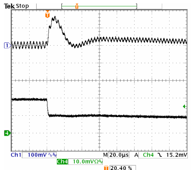
Fig-3.3V-7: Output voltage response for Vout=3.3V to negative load current step-change from 20A to 10A with slew rate of -5A/ \mu s at Vin=5.0V. Co=47 \mu Fx4 ceramic.
