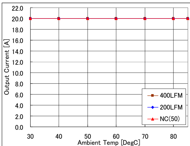
Fig-1.2V-1a: Available load current vs. ambient temperature and airflow rates for Vout=1.2V with Vin=5.0V. Maximum component temperature \leq 120^{\circ}\text{C}
