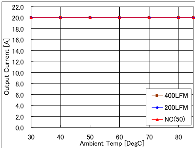
Fig-1.8V-1a: Available load current vs. ambient temperature and airflow rates for Vout=1.8V with Vin=5.0V. Maximum component temperature \leq 120^{\circ}\text{C}
