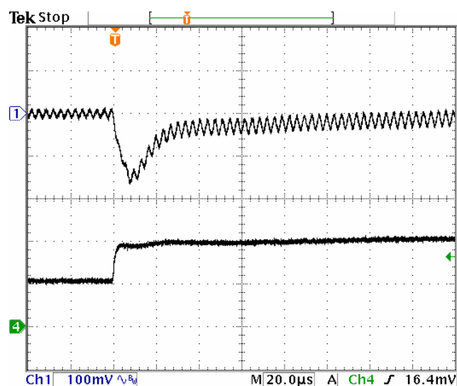
Fig-1.8V-6: Output voltage response for Vout=1.8V to positive load current step-change from 10A to 20A with slew rate of 5A/ \mu s at Vin=5.0V. Co=47 \mu Fx4 ceramic.
