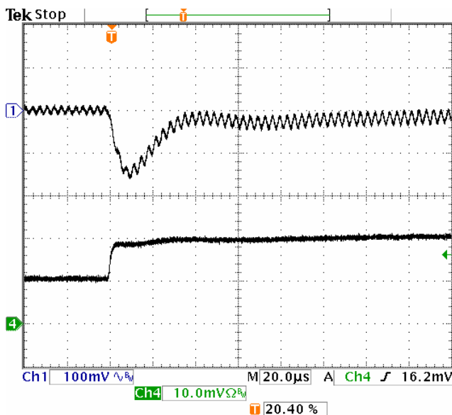
Fig-1.5V-6: Output voltage response for Vout=1.5V to positive load current step-change from 10A to 20A with slew rate of 5A/ \mu s at Vin=5.0V. Co=47 \mu Fx4 ceramic.
