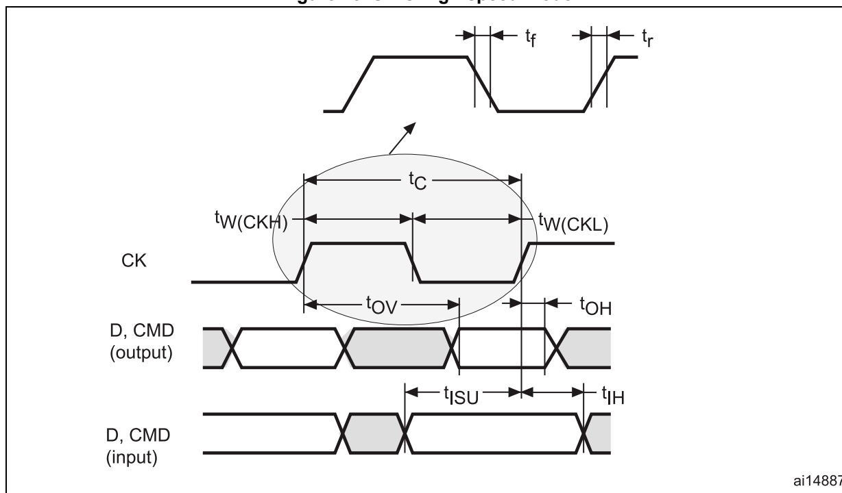
Figure 73. SDIO high-speed mode
