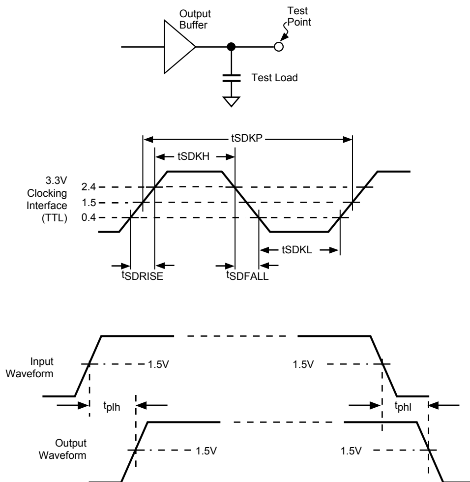
Figure 1. Clock Waveforms
