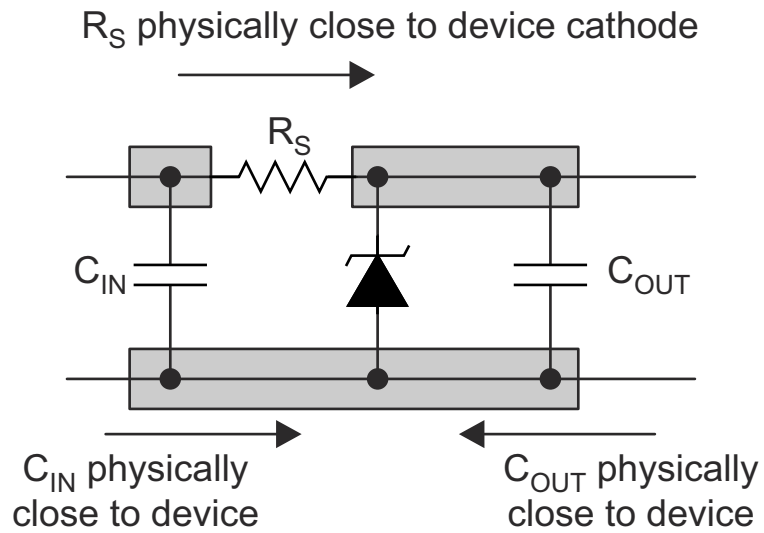
Figure 8-9. Layout Diagram
