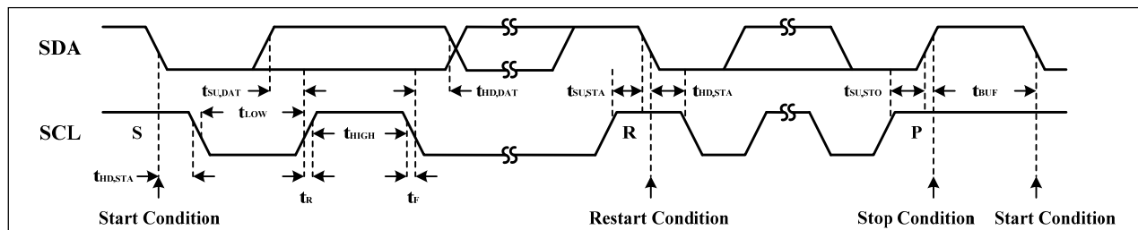
Figure 13 Interface timing
