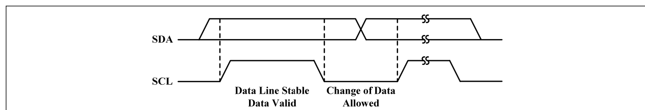
Figure 14 Bit transfer
