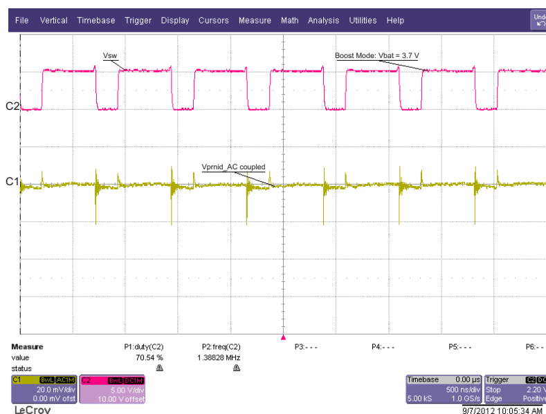
Figure 5. Boost Mode Ripple and Duty Cycle; V_{BAT} = 3.7\text{ V}
