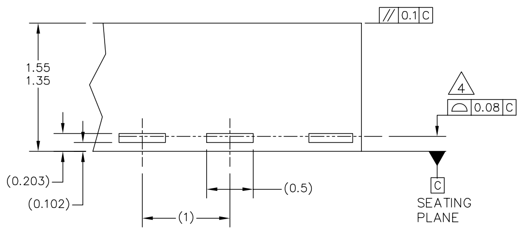
DETAIL M
