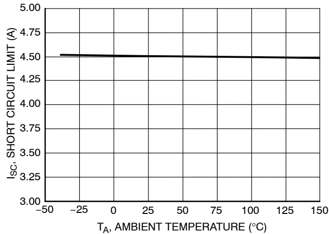
Figure 5. Short Circuit Current Limit vs. Ambient Temperature
