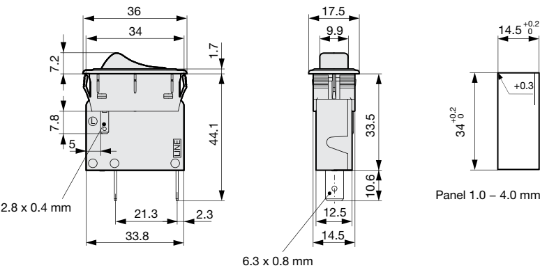
1-pole, 1 bimetal, non illuminated
