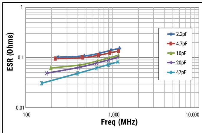
ESR vs. Frequency 0603
