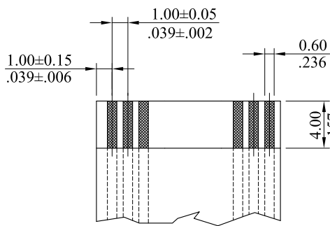
Recommended FFC/FPC Pattern Thickness 0.3mm (.012")
