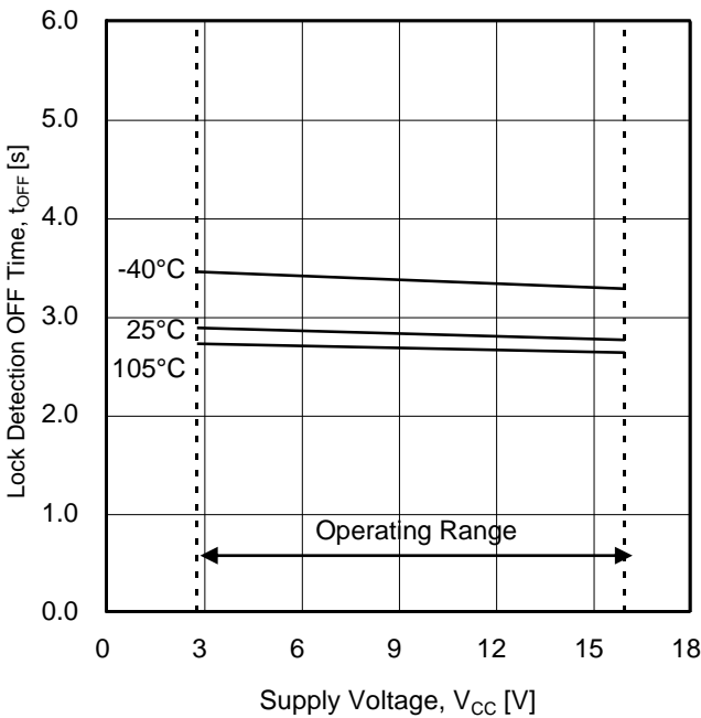
Figure 12. Lock Detection OFF Time
