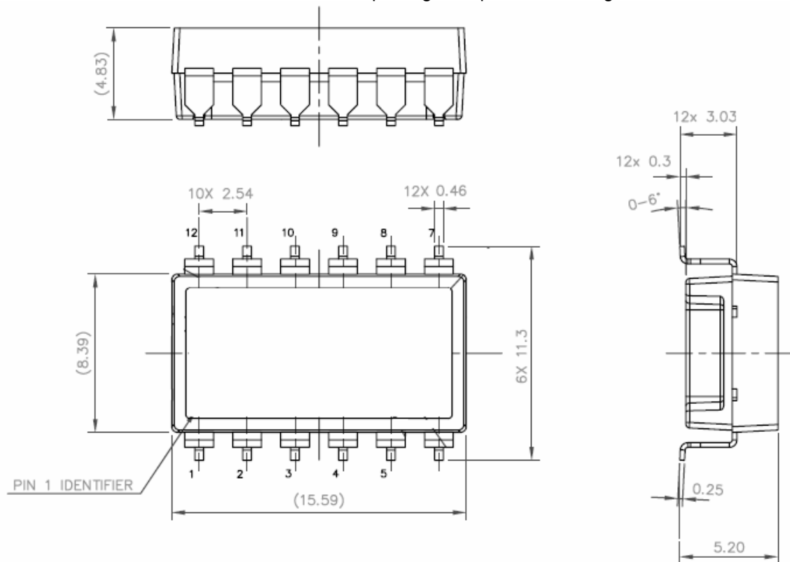
Figure 3: Outline and dimensions for DIL-12 package.
