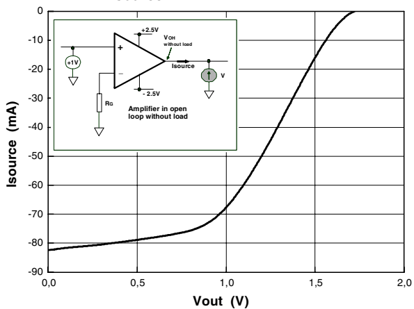
Figure 42. I_{source}
