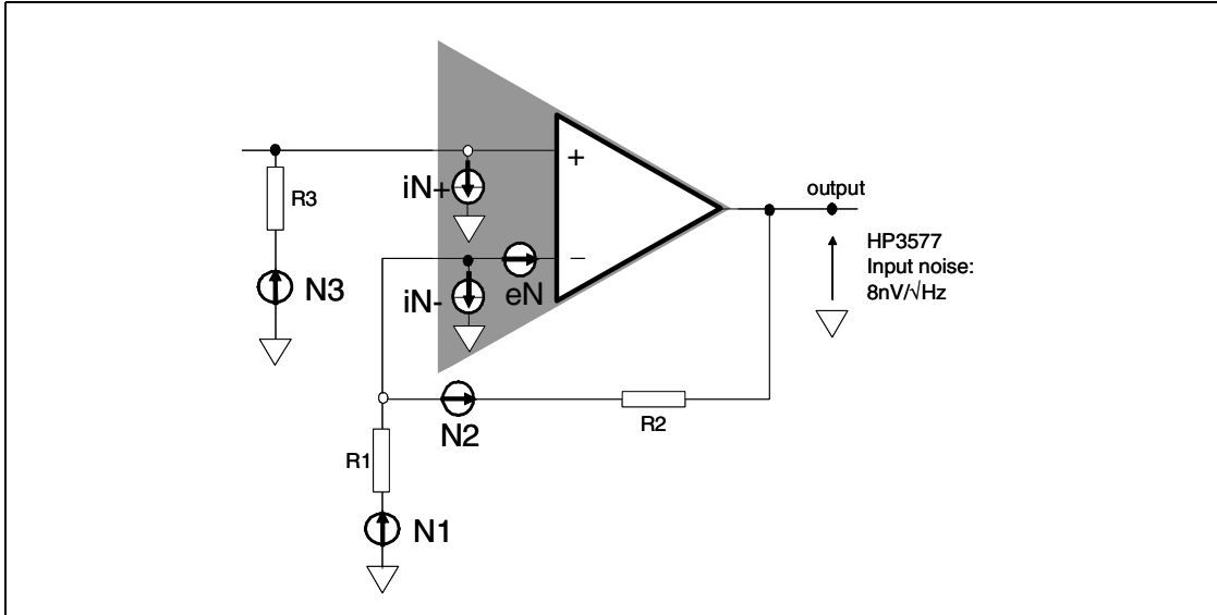
Figure 45. Noise model
