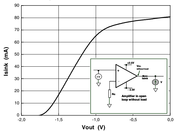
Figure 40. I_{sink}
