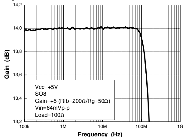
Figure 13. Gain flatness, G=+5 , SO8
