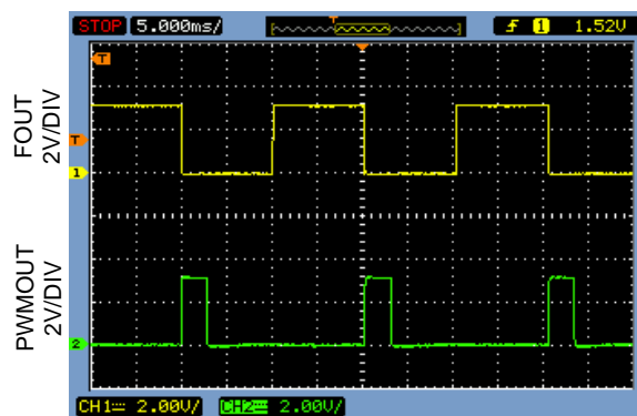
FOUT and PWMOUT V_{DD} = 3V , C_{LOAD} = 15pF , V_{PWM\_CNTRL} = V_{DD} , C_{PWM} = 10nF
