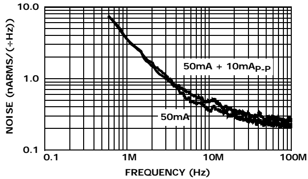
FIGURE 9. I_{\text{BLUE}} NOISE vs FREQUENCY
