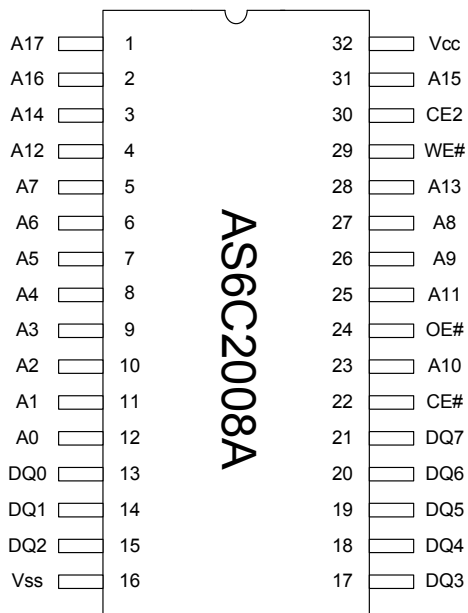
SOP/P-DIP
