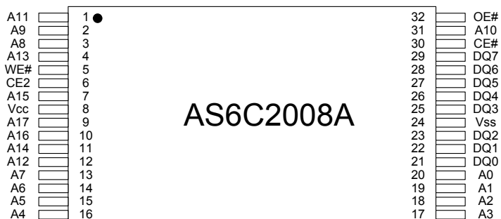
TSOP-I/STSOP
