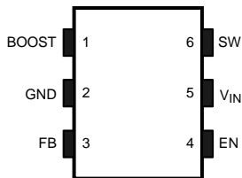
Pin Functions
