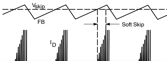
Figure 36. Soft-Skip Operation
