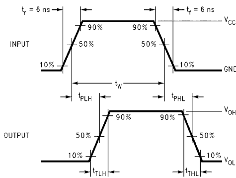
FIGURE 3. AC Waveforms
