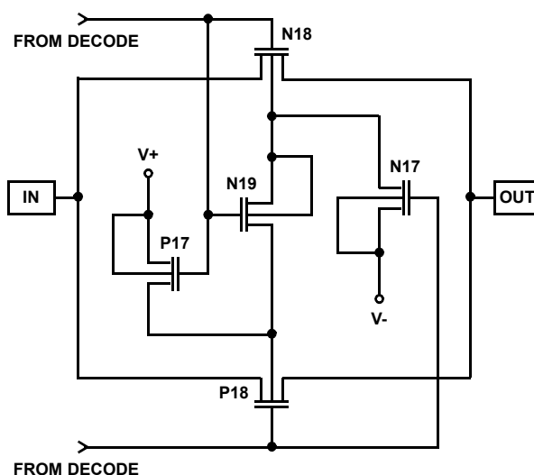
MULTIPLEX SWITCH
