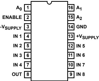
HI-508 (PDIP, CERDIP, SOIC) TOP VIEW
