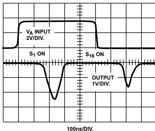
FIGURE 6C. WAVEFORMS
