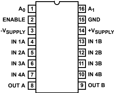
HI-509 (PDIP, Cerdip, SOIC) TOP VIEW
