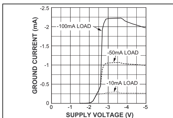
FIGURE 2-6: Ground Current vs. Input Voltage.
