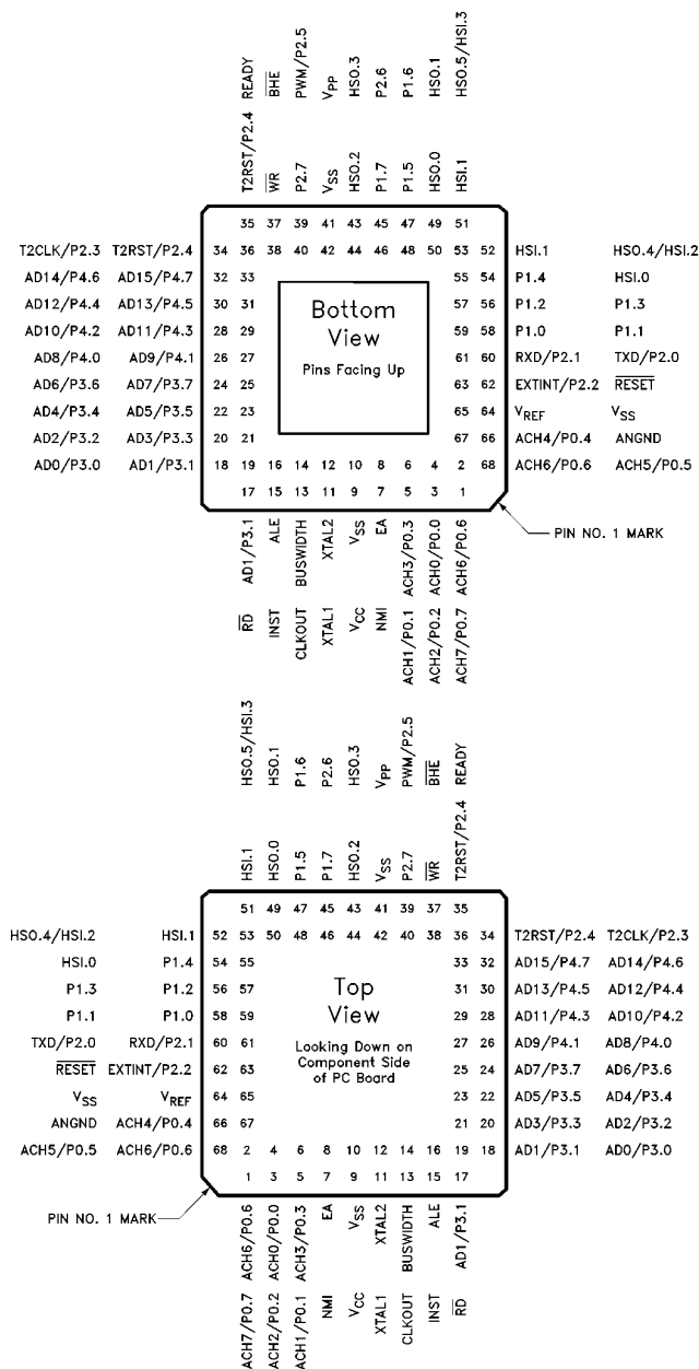
Figure 2. Pin Grid Array Pinout
