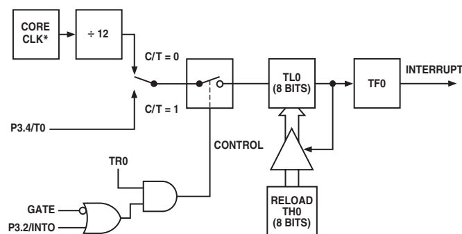
Figure 47. Timer/Counter 0, Mode 2
