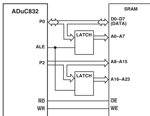
Figure 59. External Data Memory Interface (16 MBytes Address Space)
