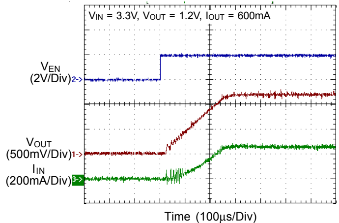
Power On
