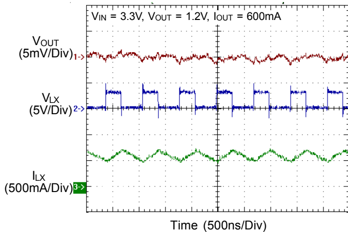
Output Ripple
