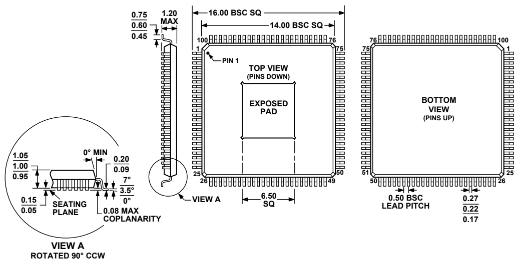
COMPLIANT TO JEDEC STANDARDS MS-026-AED-HD Figure 19. 100-Lead Thin Quad Flat Package, Exposed Pad [TQFP_EP] (SV-100-2) Dimensions shown in millimeters
