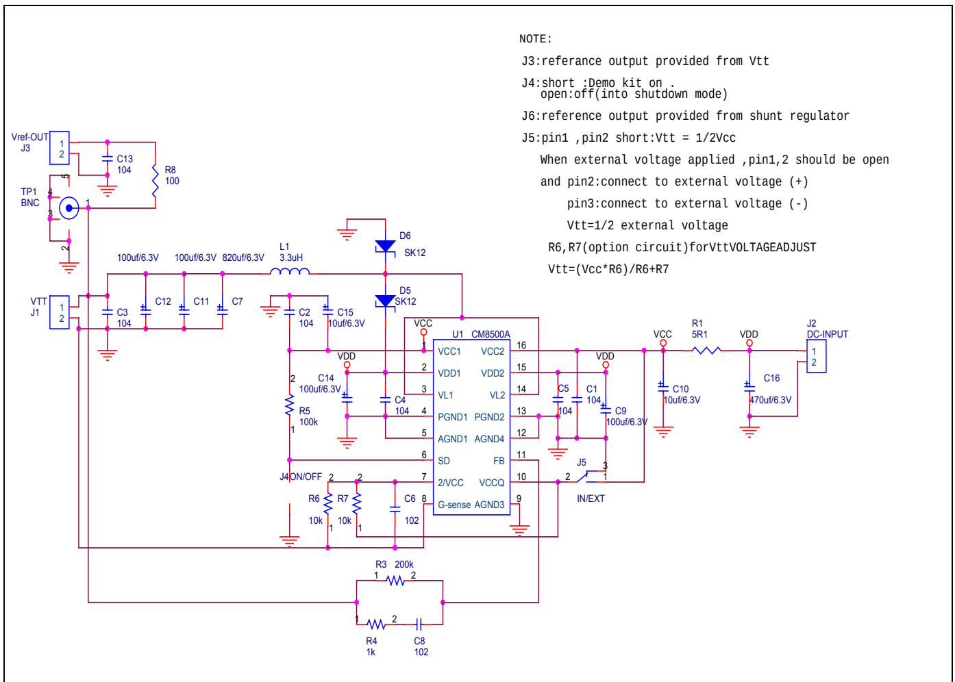
Figure 1. CM8500A Typical Application (Schematic of CM8500ATEVAL)
