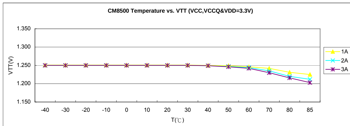
Temperature vs. VTT VCC, VCCQ & VDD=3.3V
