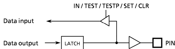
Figure 3-5. Ports P1, P2
