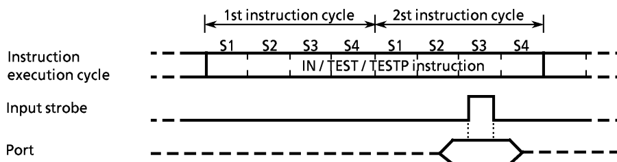
Figure 3-1. Input Timing
