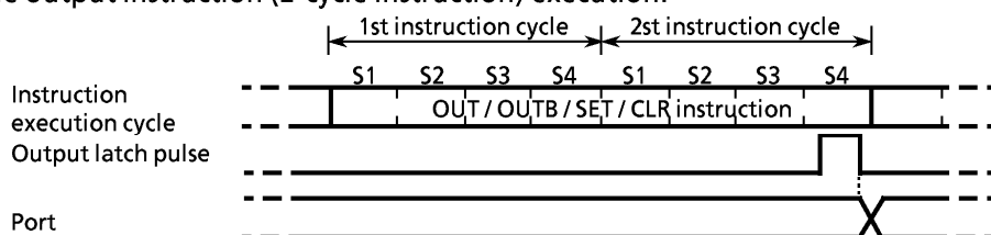
Figure 3-2. Output Timing
