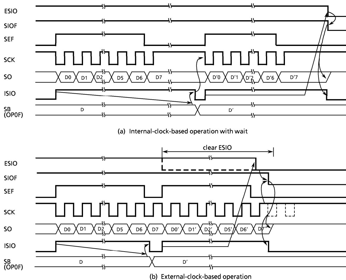
Figure 3-35. Transmit Mode
