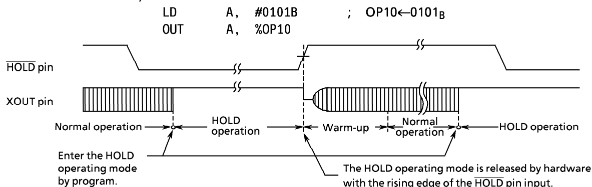
Figure 2-21. Edge-sensitive Release Mode
