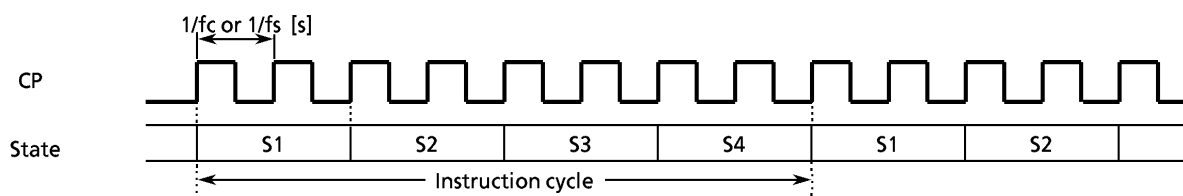
Figure 2-18. Instruction Cycle
