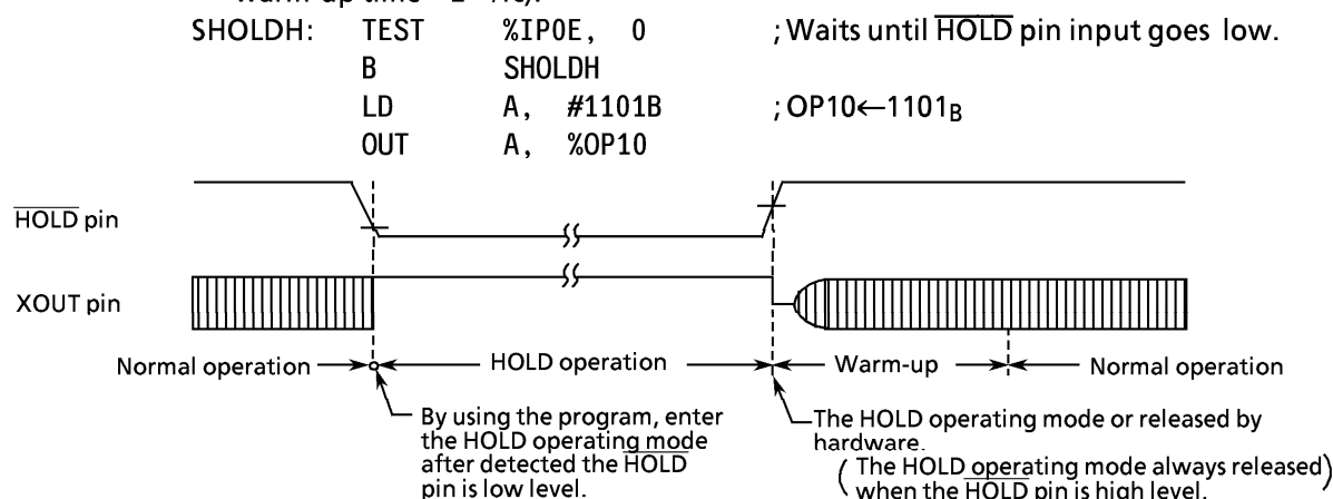
Figure 2-20. Level-sensitive Release Mode
