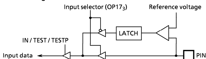
Figure 3-3. Port K0
