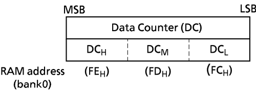
Figure 2-7. Data Counter
