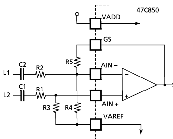
Figure 3-29. The Typical Connection for the Balance Circuit
