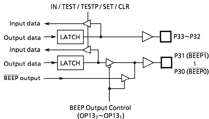
Figure 3-6. Port P3
