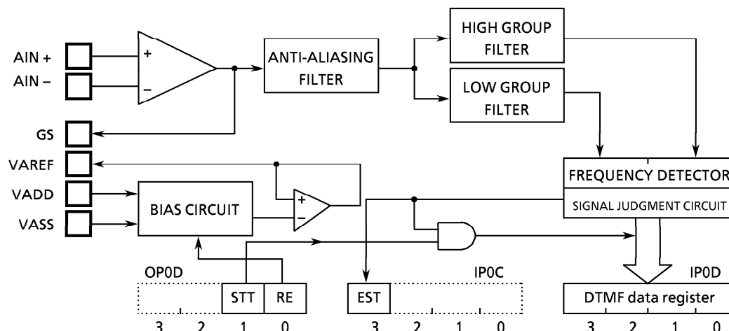
Figure 3-28. DTMF Receiver
