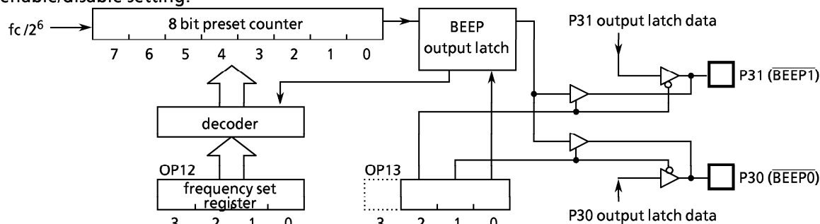
Figure 3-26. BEEP Output Circuit
