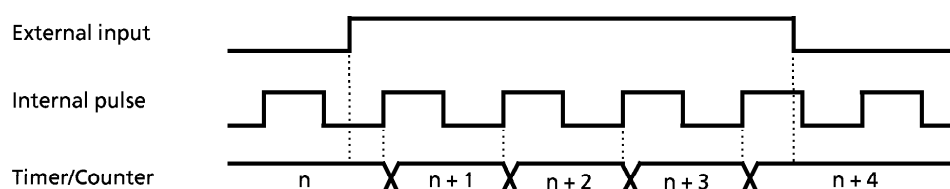
Figure 3-21. Pulse Width Measurement Mode Timing Chart
