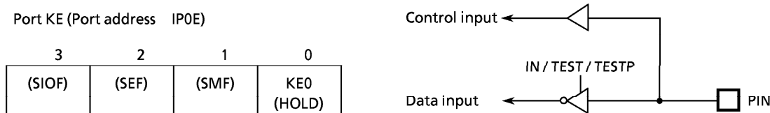
Figure 3-13. Port KE
