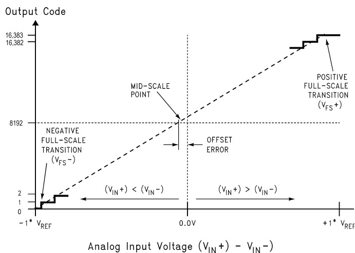
Figure 4. Transfer Characteristic
