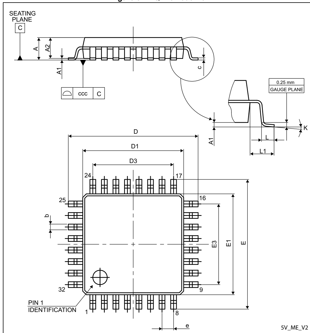
Figure 34. LQFP32 outline
