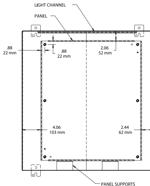
SECTION Y-Y
