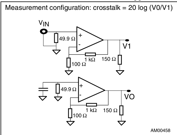
Figure 24. Channel separation (crosstalk) vs. frequency schematic ( V_{CC} = \pm 5\text{ V} )
