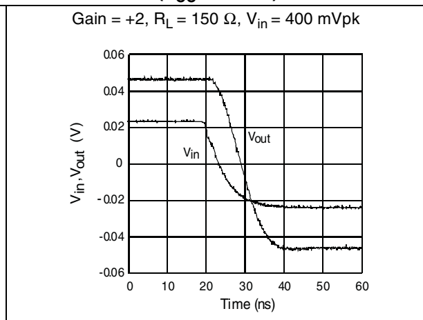
Figure 8. Small signal measurement – fall time ( V_{CC} = \pm 2.5 V)
