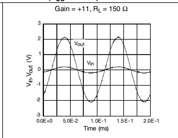
Figure 12. Maximum output swing ( V_{CC} = \pm 2.5 V)
