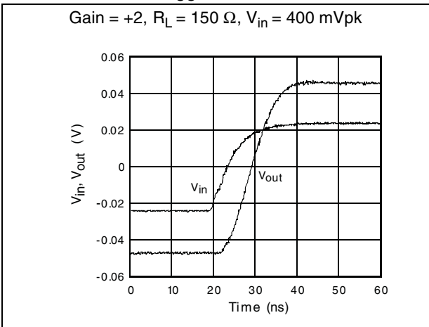
Figure 22. Small signal measurement – rise time ( V_{CC} = \pm 5\text{ V} )
