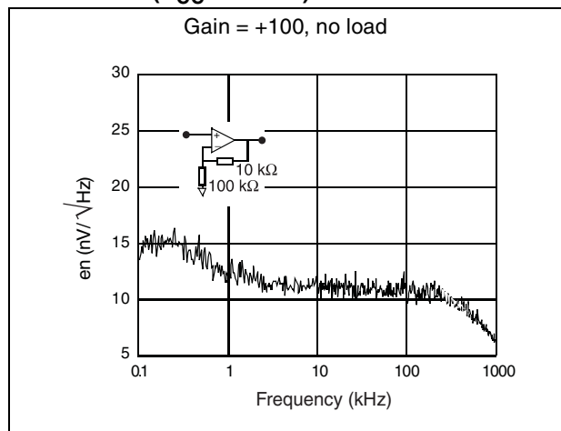
Figure 11. Equivalent input noise voltage ( V_{CC} = \pm 2.5 V)
