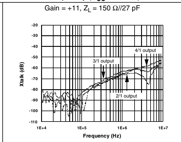
Figure 10. Channel separation (crosstalk) vs. frequency ( V_{CC} = \pm 2.5 V)
