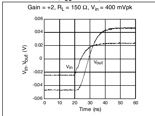
Figure 7. Small signal measurement – rise time ( V_{CC} = \pm 2.5 V)
