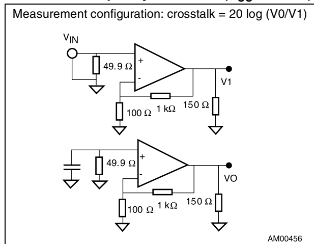
Figure 9. Channel separation (crosstalk) vs. frequency schematic ( V_{CC} = \pm 2.5 V)
