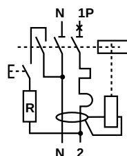
1 protected pole + switched neutral
